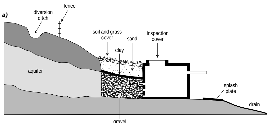
Figure 3.11. Sanitary protection measures for a) springs and b) boreholes
